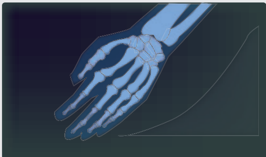
x-ray
